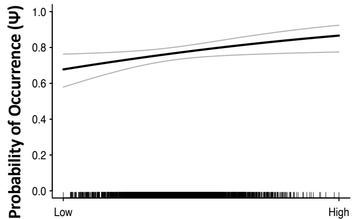
Mean Annual Rainfall
